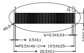
DETAIL A(2.5:1)
