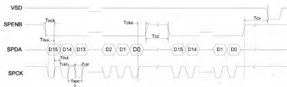
Source Driver Output Timing Diagram
