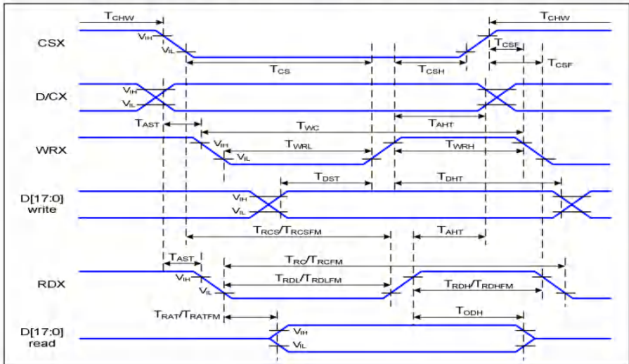
8080 Series MCU Parallel Interface Characteristics: 18/16/9/8-bit Bus
