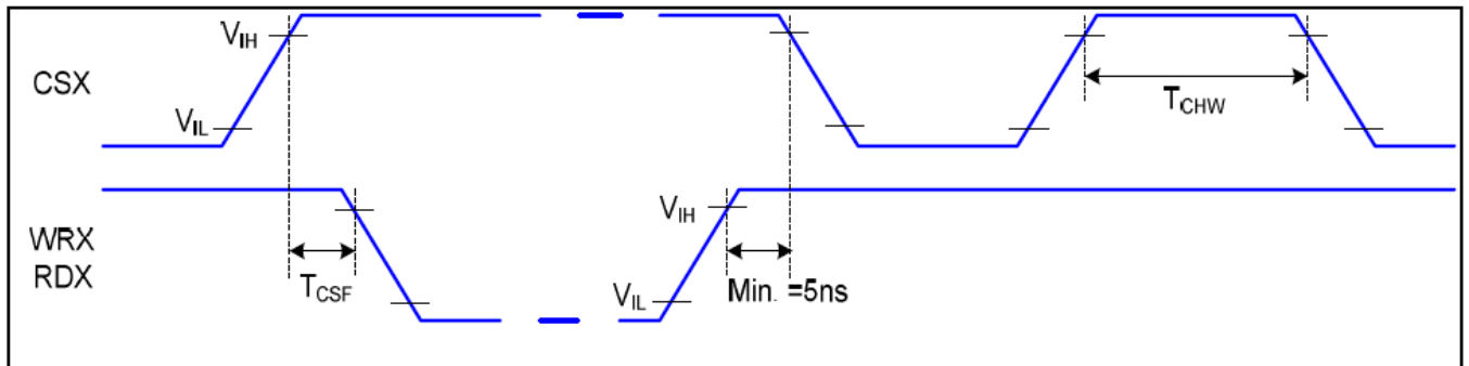
Figure 3. Chip Selection(CSB) Timing
