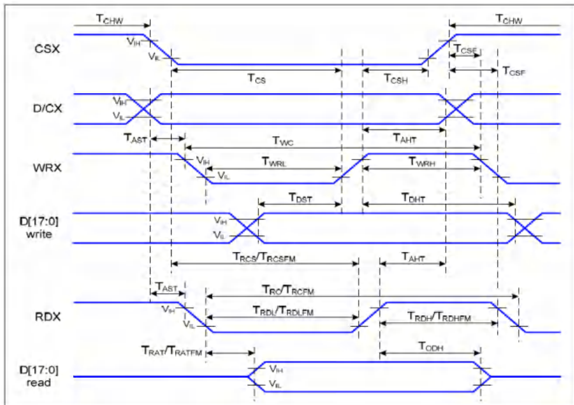
Figure 1. Parallel Interface Timing Characteristics(80-Series MCU interface)
